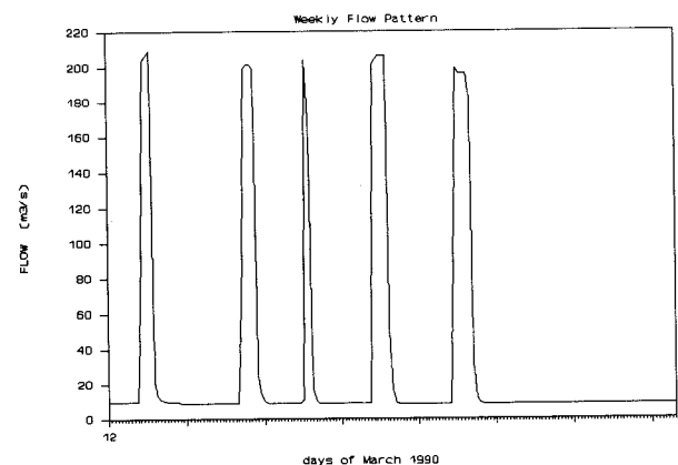
Figure 3b. Winter flow pattern with one large daily fluctuation during working days and lower base flow on weekends (after GARCIA DE JALON & SANCHEZ, in press ).
