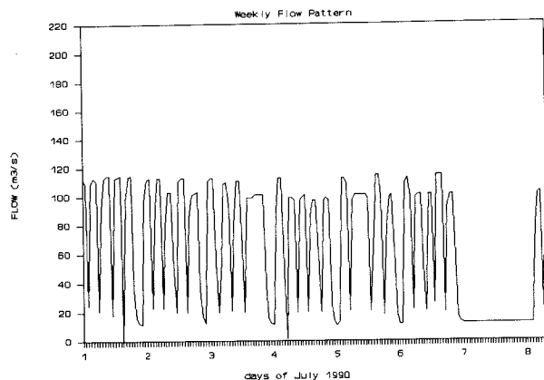
Figure 3a. Hydroelectric flow regime below Valparaíso reservoir in summer: 5 daily fluctuations during working days and larger base flow on weekends.
